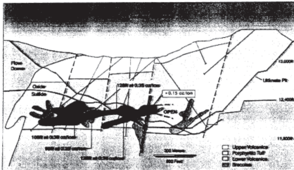
Above: Chaquicocha cross section looking northeast.
