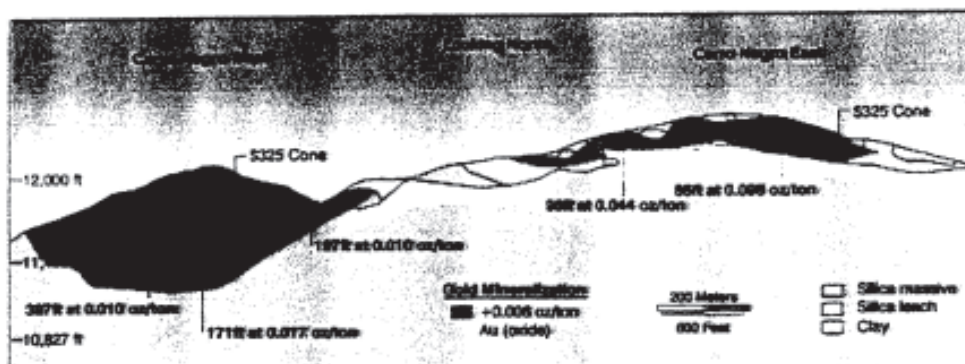
Above: Section showing the Cerro Negro West and Cerro Negro East deposits, looking north.
